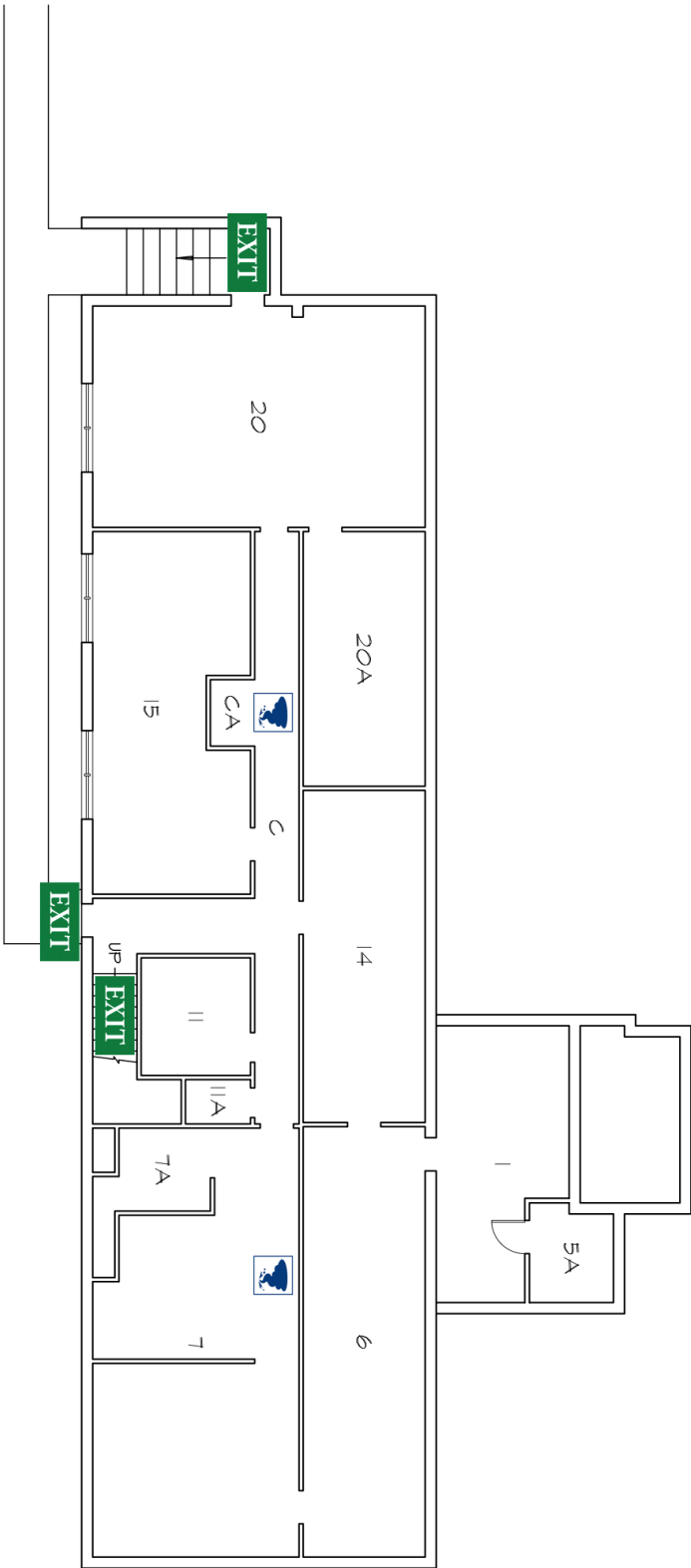
NORTH BASEMENT FLOOR PLAN 0 8 16 24 32 FEET
