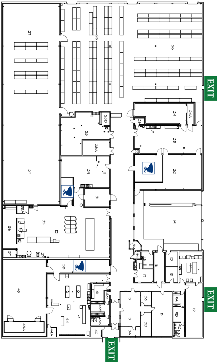
NORTH FIRST FLOOR PLAN 0 16 32 48 64 FEET
