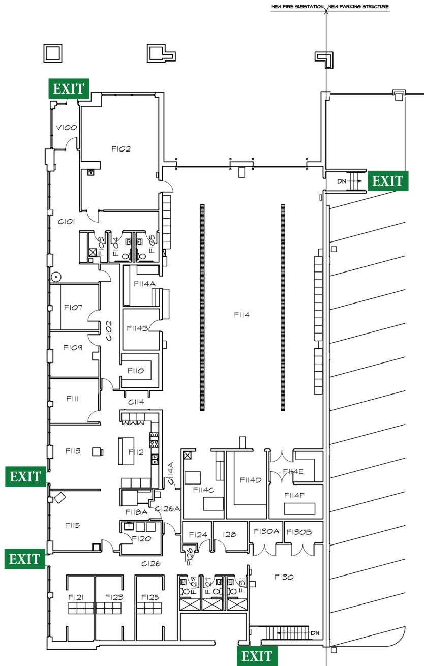
FIRST FLOOR PLAN 0 8 16 24 32 FEET
