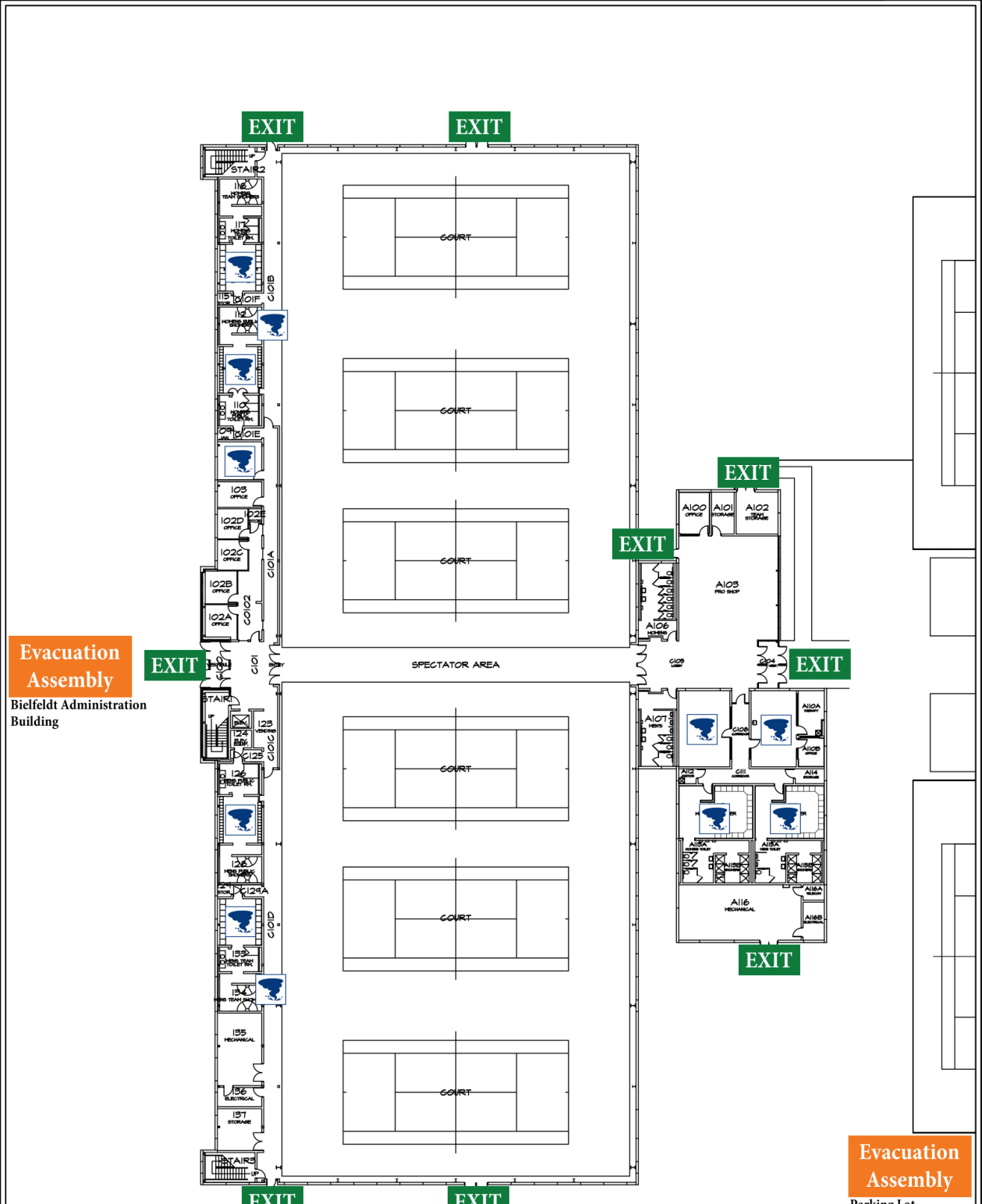
FIRST FLOOR PLAN 0 16 32 48 64 FEET
